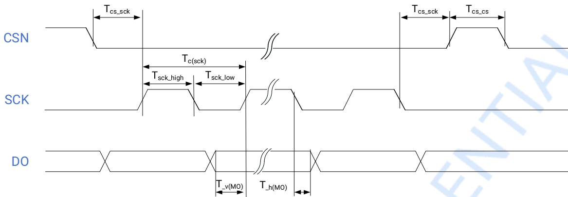
Figure 8-12 Data communication SPI timing diagram – master mode
