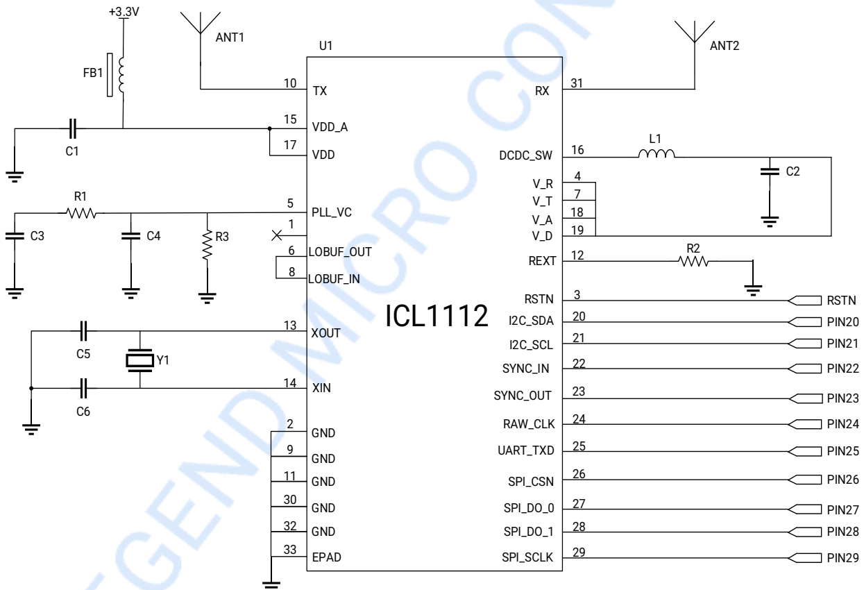
Figure 9-1 mmWave sensor application schematic
