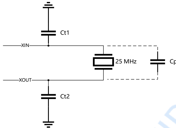
Figure 7-3 Crystal implementation
